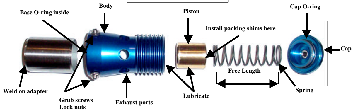
Figure 1 Exploded View of the BOV I
